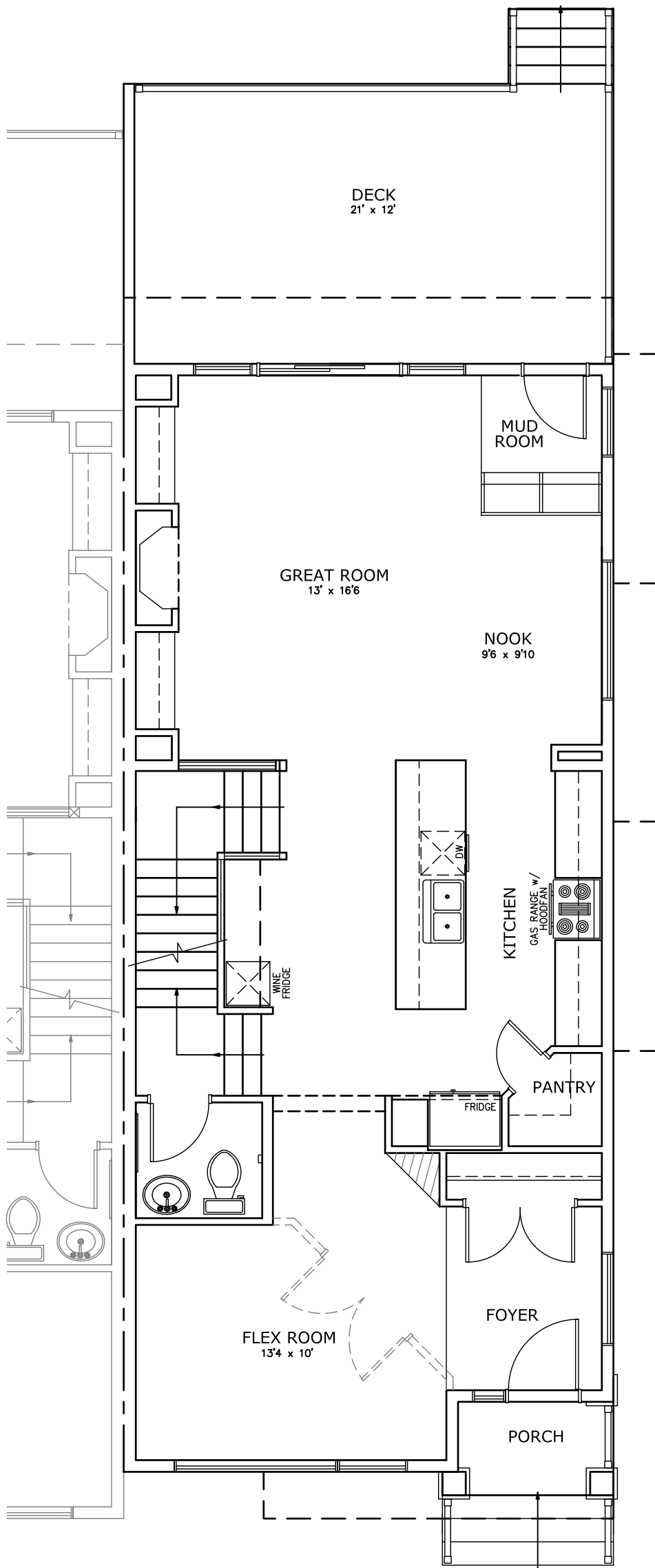
MAIN FLOOR 978 sqft.
